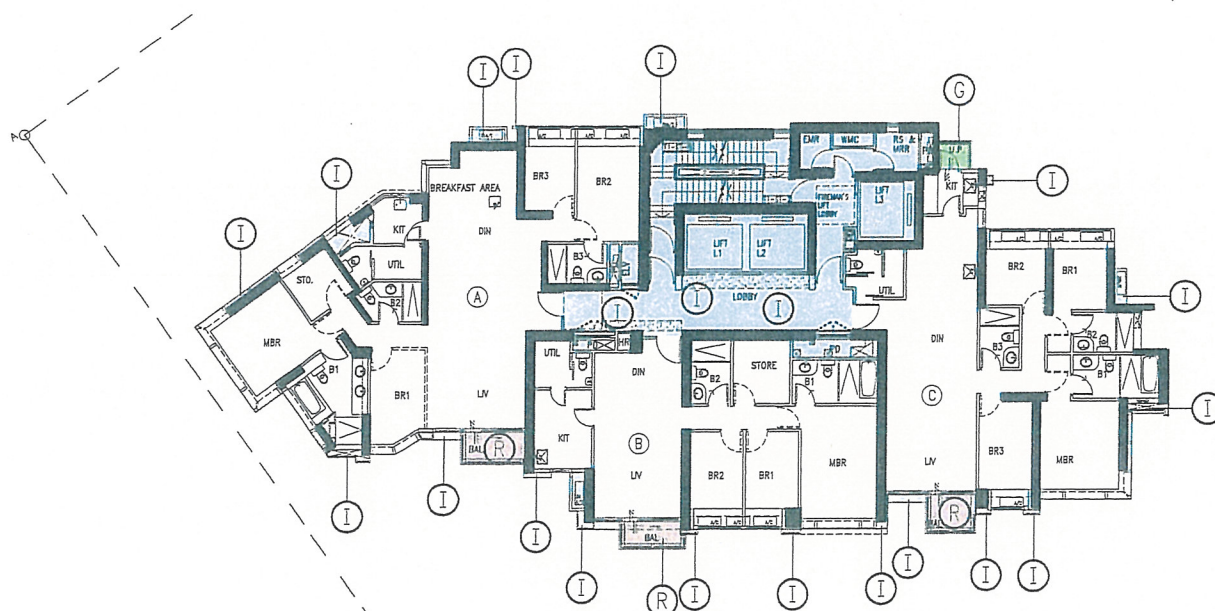
TOWER 1 7TH TO 37TH FLOOR PLAN (14/F, 24/F & 34/F OMITTED)
