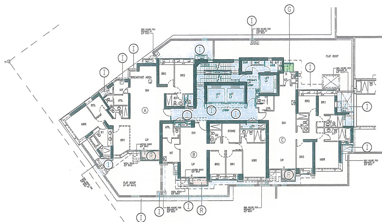
TOWER 1 6TH FLOOR PLAN
