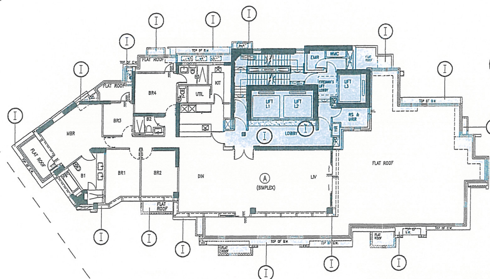
TOWER 1 38TH FLOOR PLAN (PRESIDENTIAL FLOOR 1)
