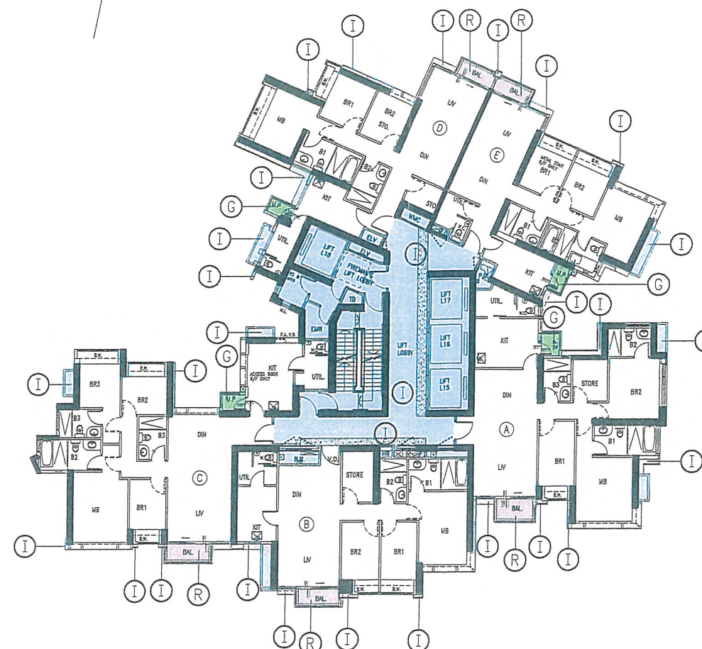
TOWER 8 15TH FLOOR PLAN - REFUGE FLOOR
